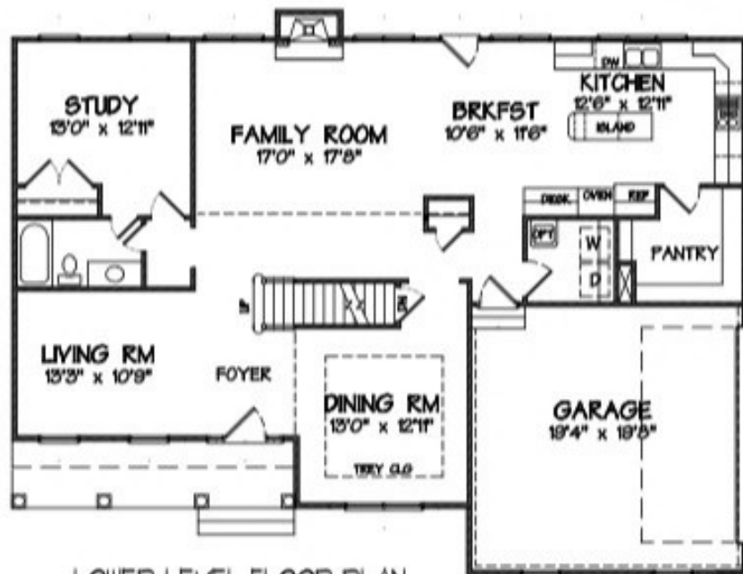
LOWER LEVEL FLOOR PLAN
